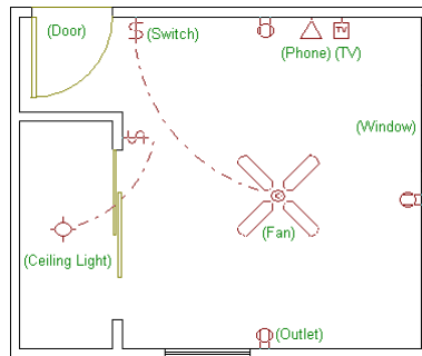
Circuit: "SE Bedroom" 15 A Your Plan
